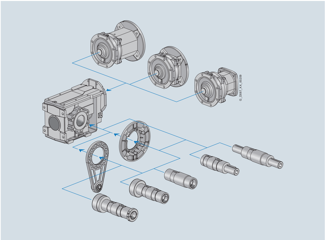
Fig. 1/12 Modular system, bevel gearbox B
