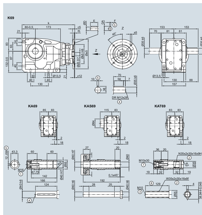
Fig. 1/16 Example, dimensional drawing
