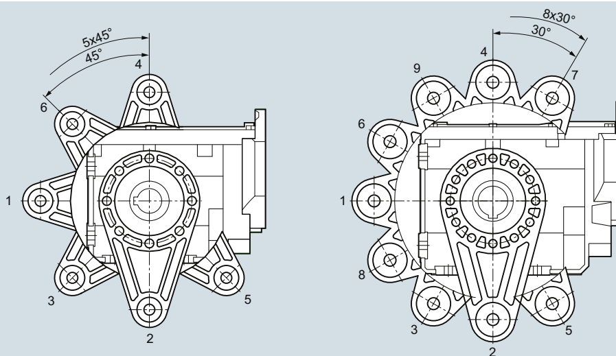
Fig. 9/8 Bevel gearboxes B in a shaft-mounted design
